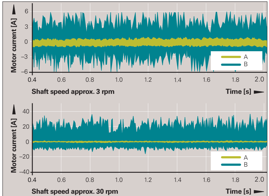
Motor current of a direct drive with position encoder A: With low interpolation error (optical encoder) B: With high interpolation error (magnetic encoder)
