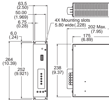
Dimensions in mm (inches)
