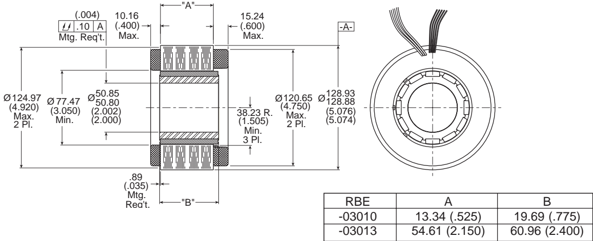
Dimensions in inches (mm)
