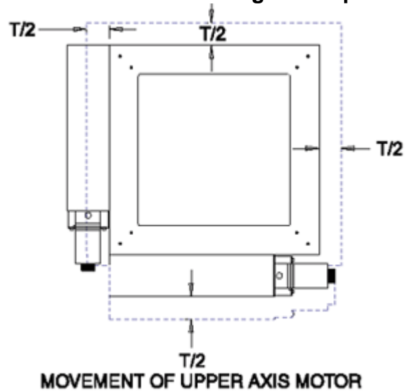
Dimensions - Moving Envelope
