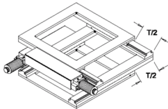
Dimensions - Perspective
