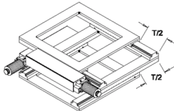
Dimensions - Perspective
