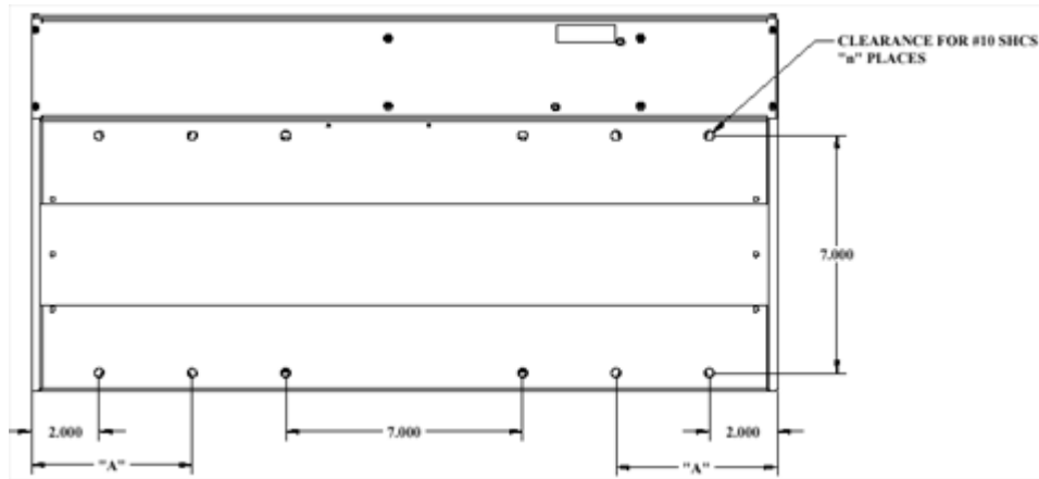
Dimensions - Bottom View
