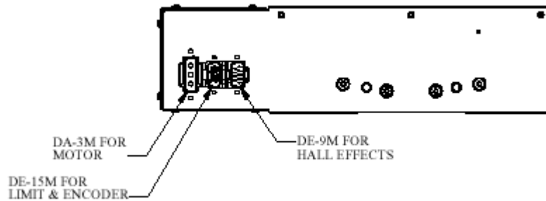
Dimensions - End View
