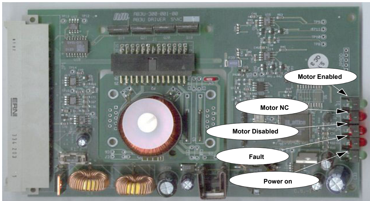
Figure 8: LED Indicators
