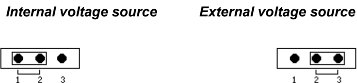
Figure 6: Jumper 2 Configuration
