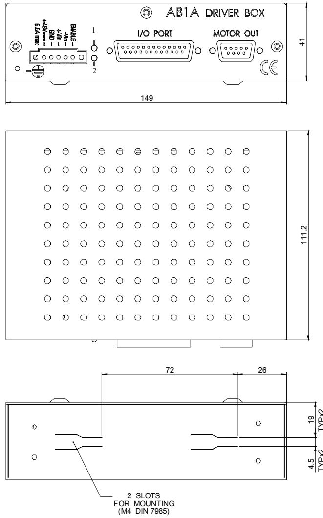
Figure 9: AB1A Layout
