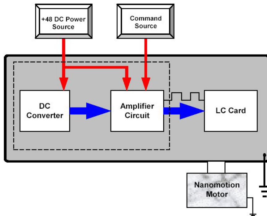
Figure 1: AB1A Block Diagram
