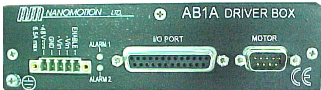
Figure 3: AB1A Driver Box Front Panel
