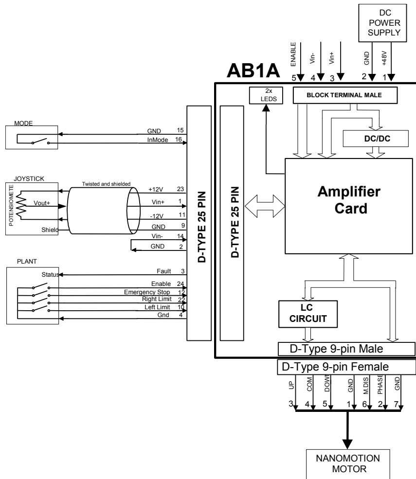
Figure 6: Joystick Connection
