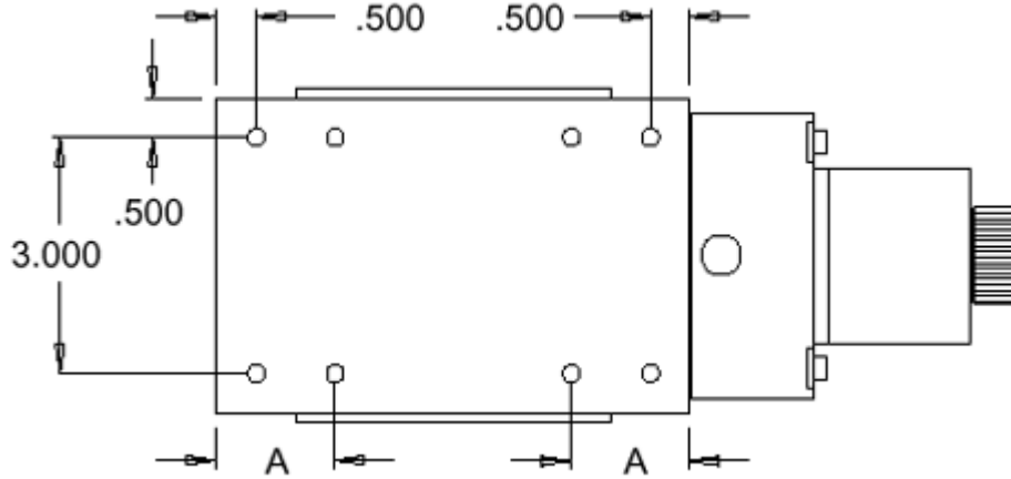
Dimensions - Bottom View
