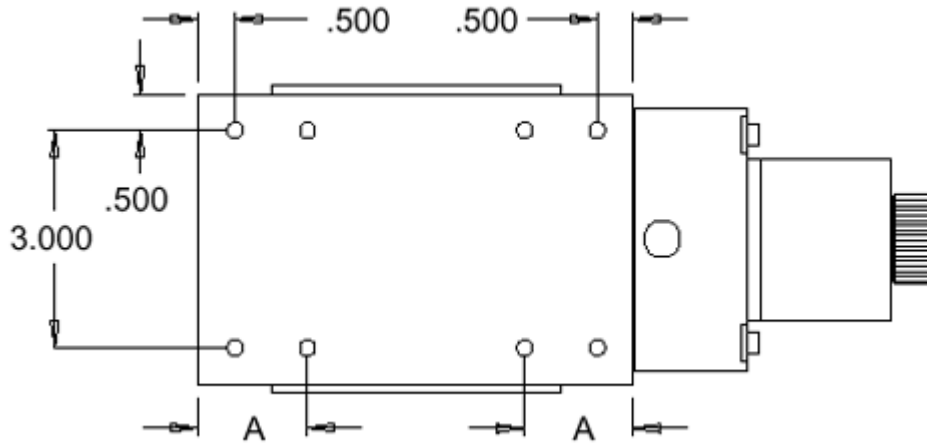
Dimensions - End View
