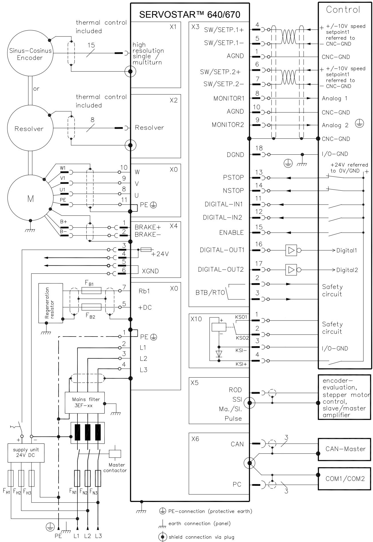
Wiring diagram SERVOSTAR™
